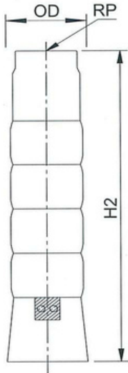
DIMENSIONS & WEIGHT
